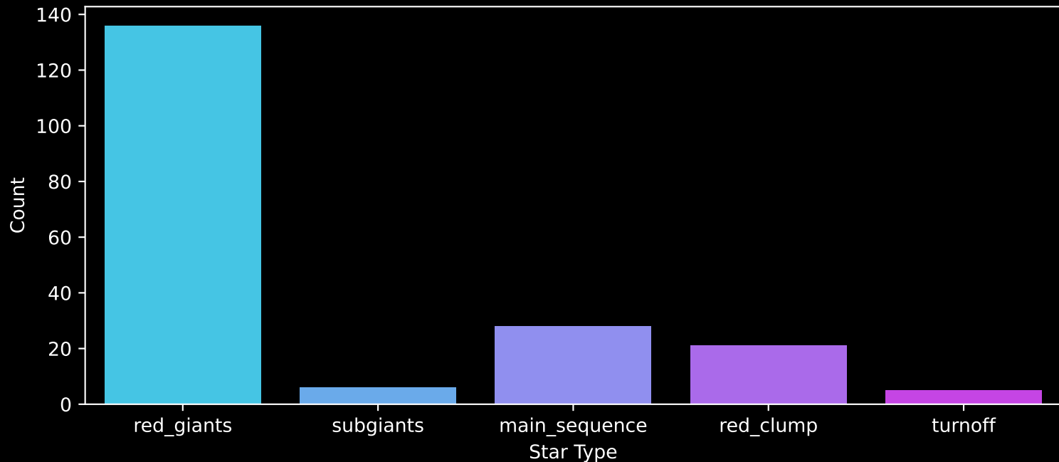
APOGEE DR17 Field: [K2_C2_352+12_btx] Count plot of Star Type
