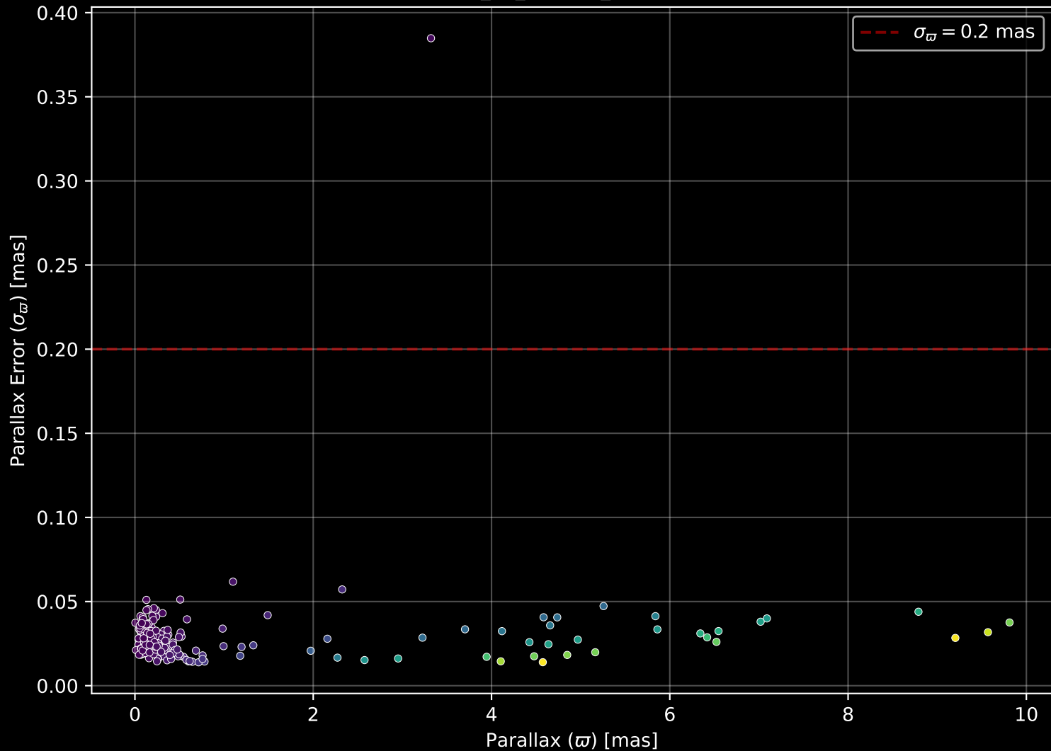
APOGEE DR17 Field: [K2_C2_352+12_btx] Parallax Quality (n= 196)
