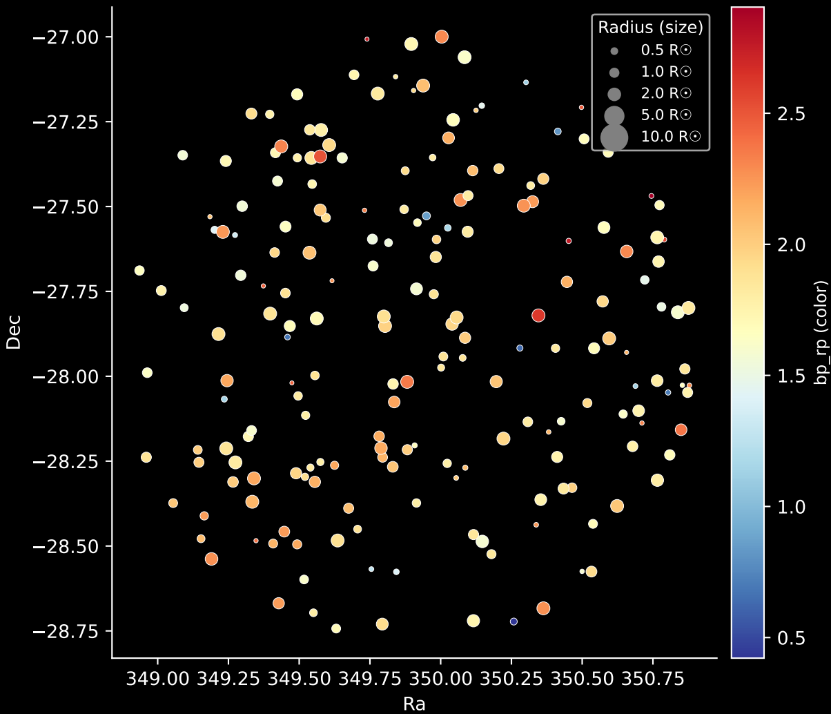
APOGEE DR17 Field: [K2_C2_352+12_btx] Stars: 196
