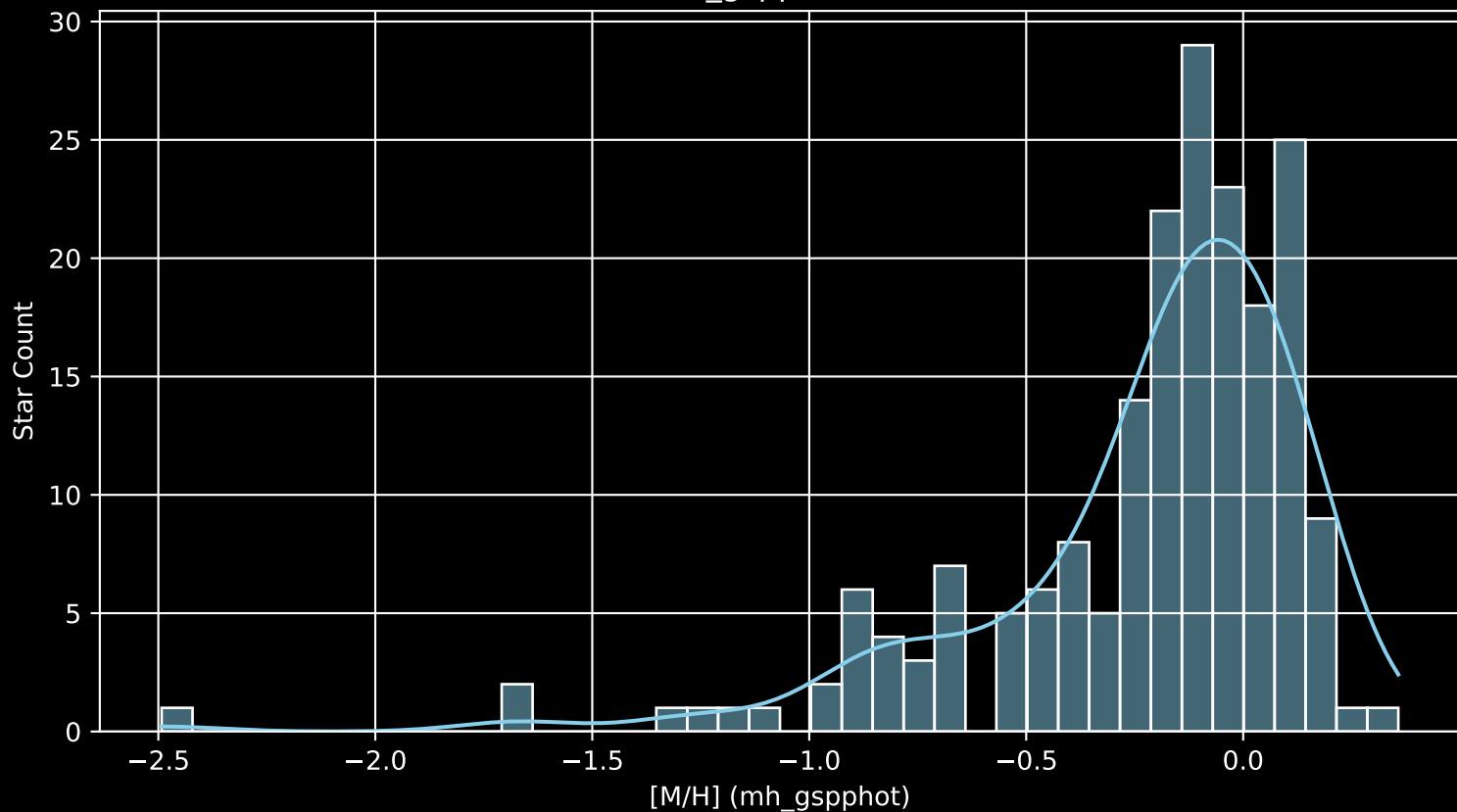
APOGEE DR17 Field: [K2_C2_352+12_btx [M/H] (mh_gspphot) (n= 195)
