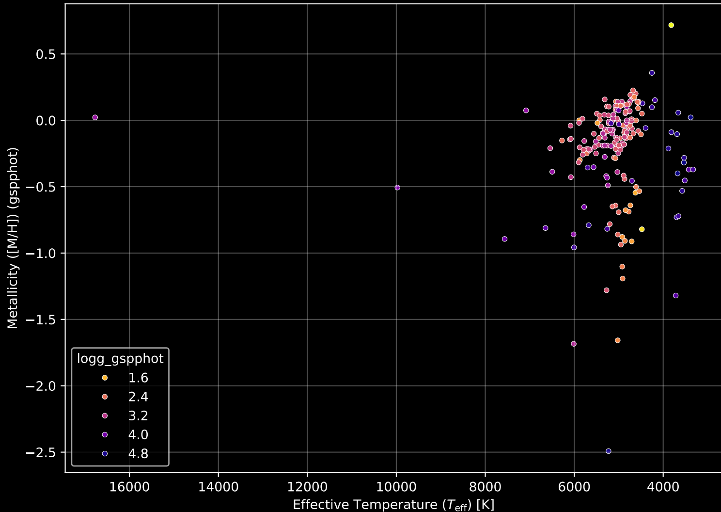
APOGEE DR17 Field: [K2_C2_352+12_btx] Stellar Population Parameters (n= 196)
