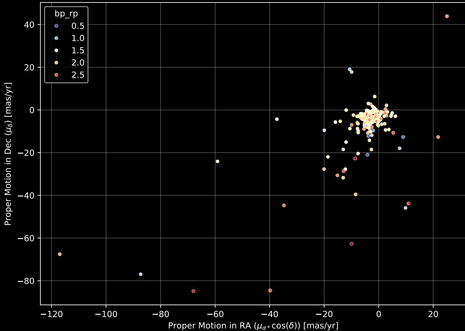
APOGEE DR17 Field: [K2_C2_352+12_btx] Proper Motion Diagram (n= 196)
