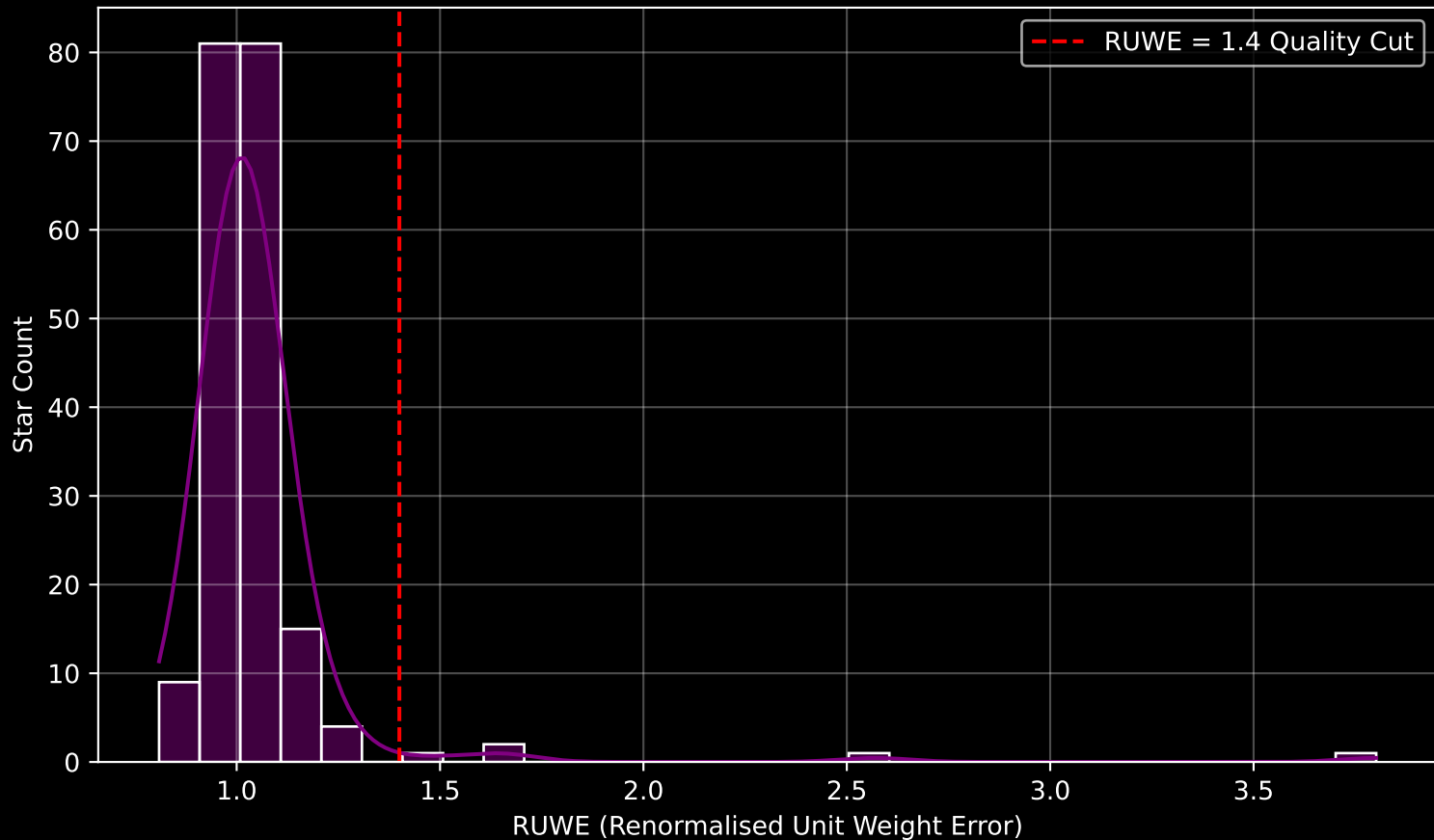
GAPOGEE DR17 Field [K2_C2_352+12_btx] RUWE Distribution (n= 195)
