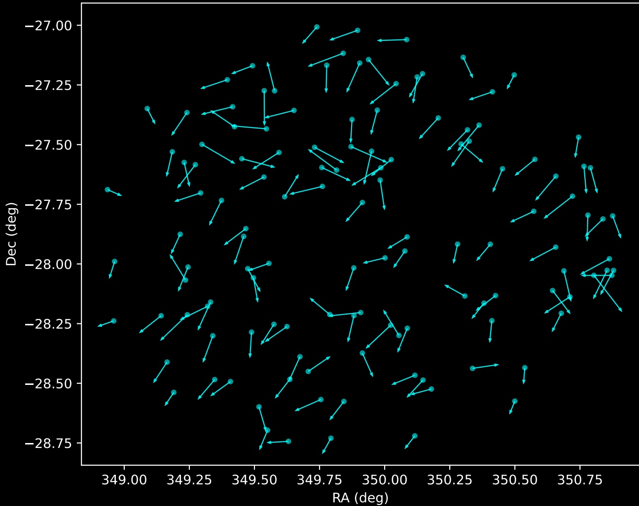
APOGEE DR17 Noise Stream Proper Motion Vectors (n=127)
